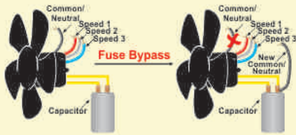
Fuse Bypass Diagram
